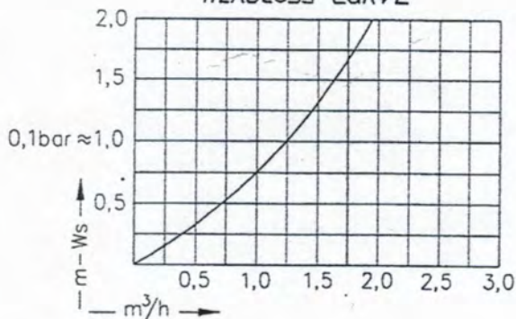
HEADLOSS CURVE
